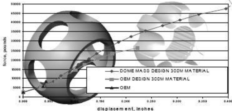
638-0 CAGE ULTIMATE STRENGTH TEST RESULTS
